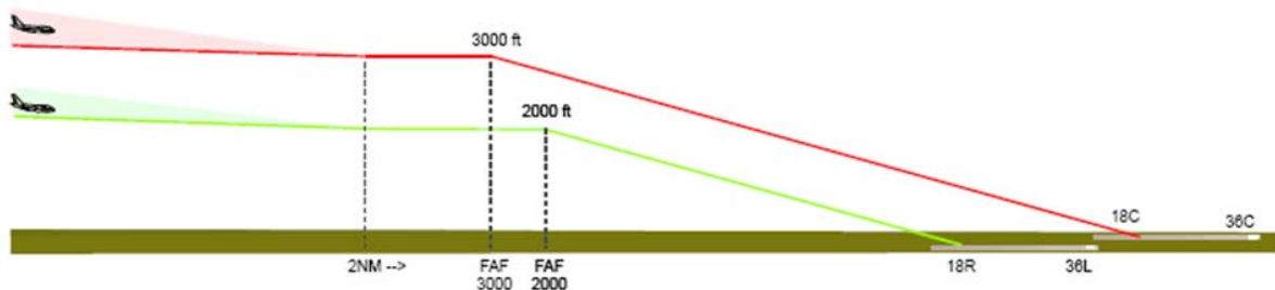
Figure 14 Illustration of vertical separation during parallel arrivals runway operations
